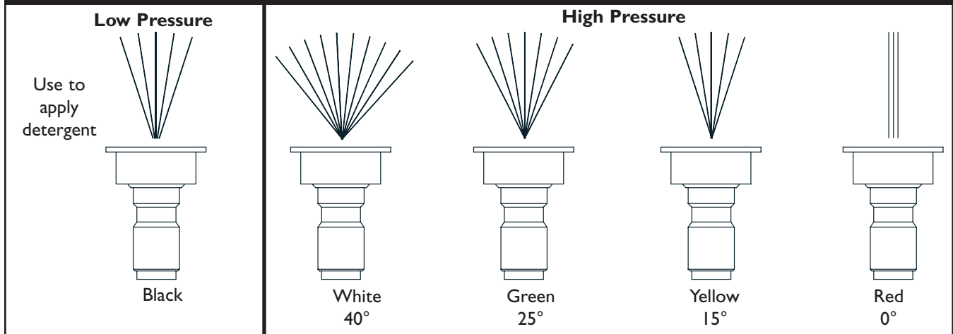
Figure 9 — Spray Tips
